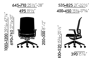
AM Chair with 3D armrests
