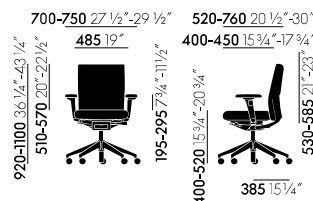
ID Soft with 2D armrests
