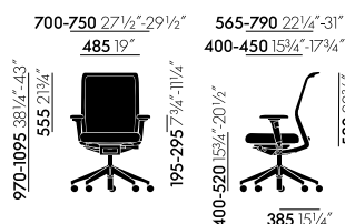
ID Mesh with 2D armrests
