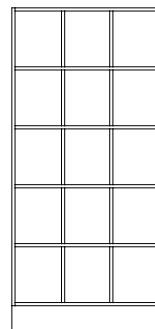
KBH90/5 898x1936x370
