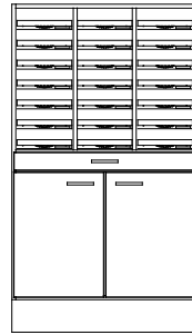
LPS3/21 898x1584x370
