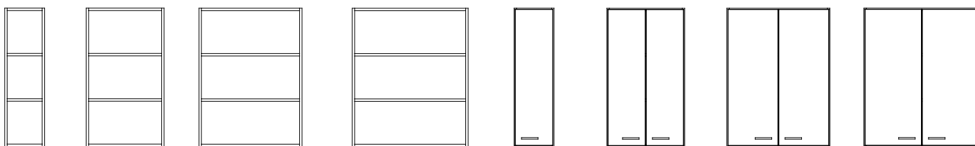
VH30/3 312x1075x370 VH60/3 605x1075x370 VH80/3 800x1075x370 VH90/3 898x1075x370
