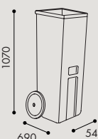
W0012 Rullkärl 190 liter W0112 Lock till 190 liter
