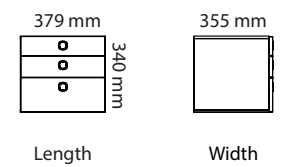
Drawer cassette
