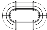
2xMES120AVH, 4xMES90Y L3120 W1920 innermätt inner L1850 W650
