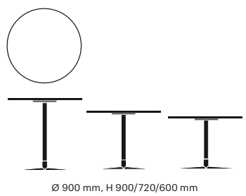
Ø 900 mm, H 900/720/600 mm
