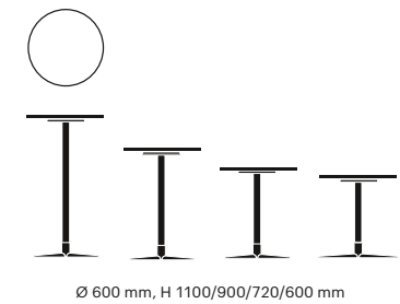
Ø 600 mm, H 1100/900/720/600 mm
