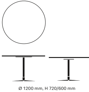
Ø 1200 mm, H 720/600 mm
