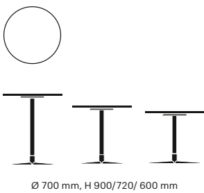
Ø 700 mm, H 900/720/600 mm
