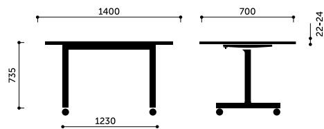
u-Connect 3490-38
