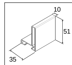
Monteringsram, profil.
