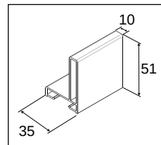
Monteringsram, profil.
