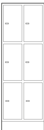
SD6/19 1932x613x580
