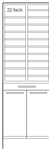
PS6/19 1932x610x372
