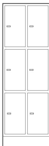
SDF6/19 1932x613x372
