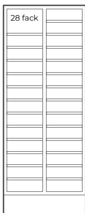
BS6/15 1580x613x372
