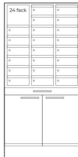
PL9/19 1932x910x372
