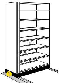
1. Ramp, aluminium
